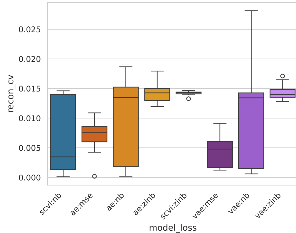
Reconstruction CV
