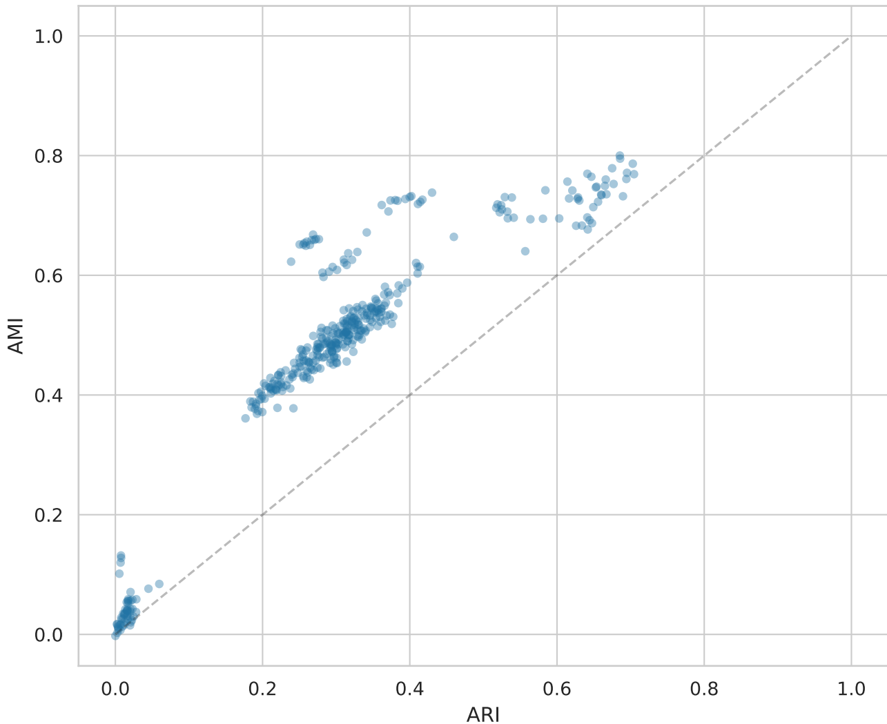
ARI vs AMI Agreement (Spearman r=0.909 )
