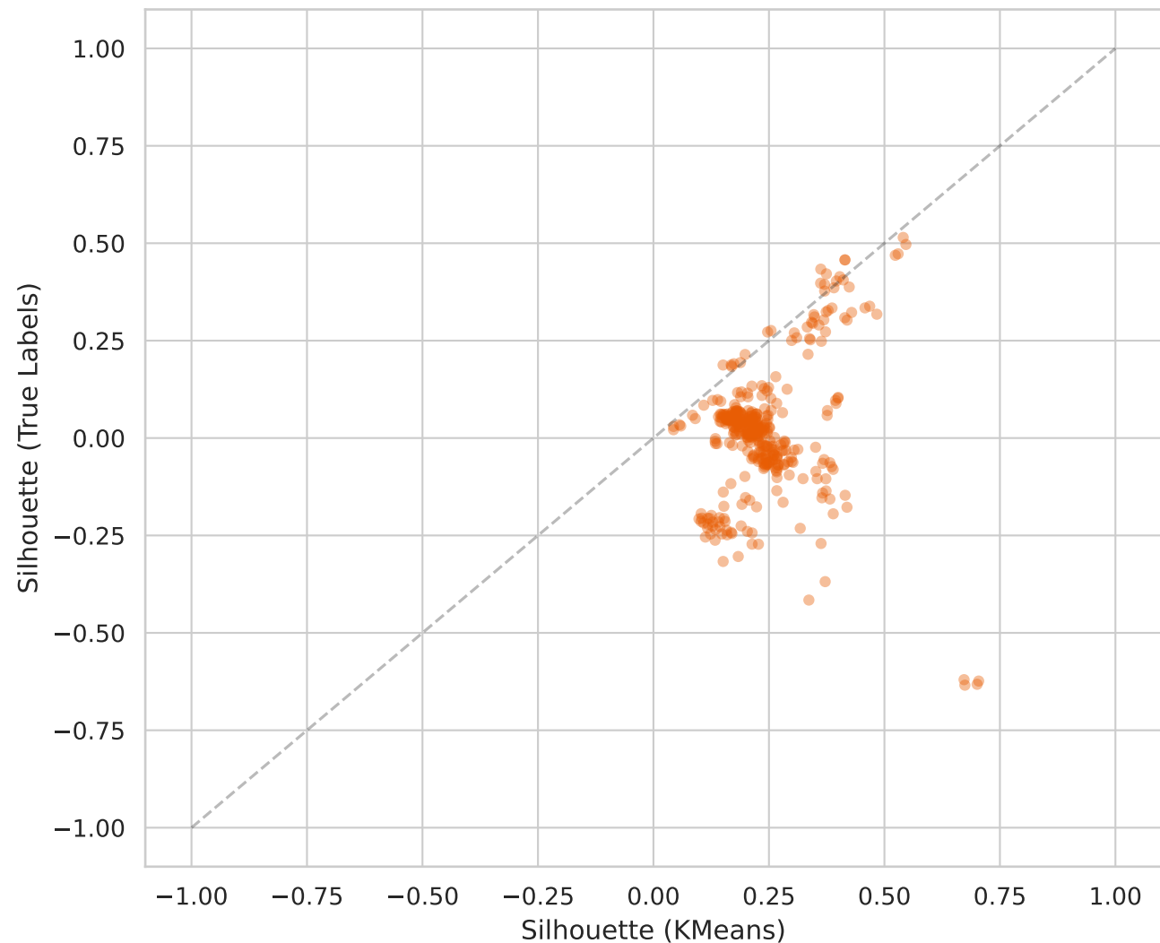
KMeans vs True-Labels Silhouette ( r=0.088 )
