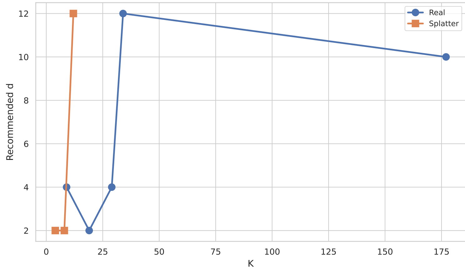
Synthetic vs Real Data: d = f(K) Comparison (scvi:nb)
