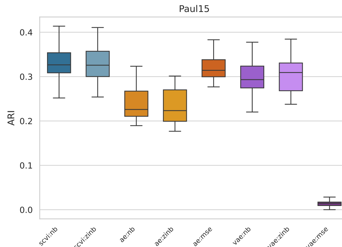
ARI Distribution by Model/Loss per Dataset
