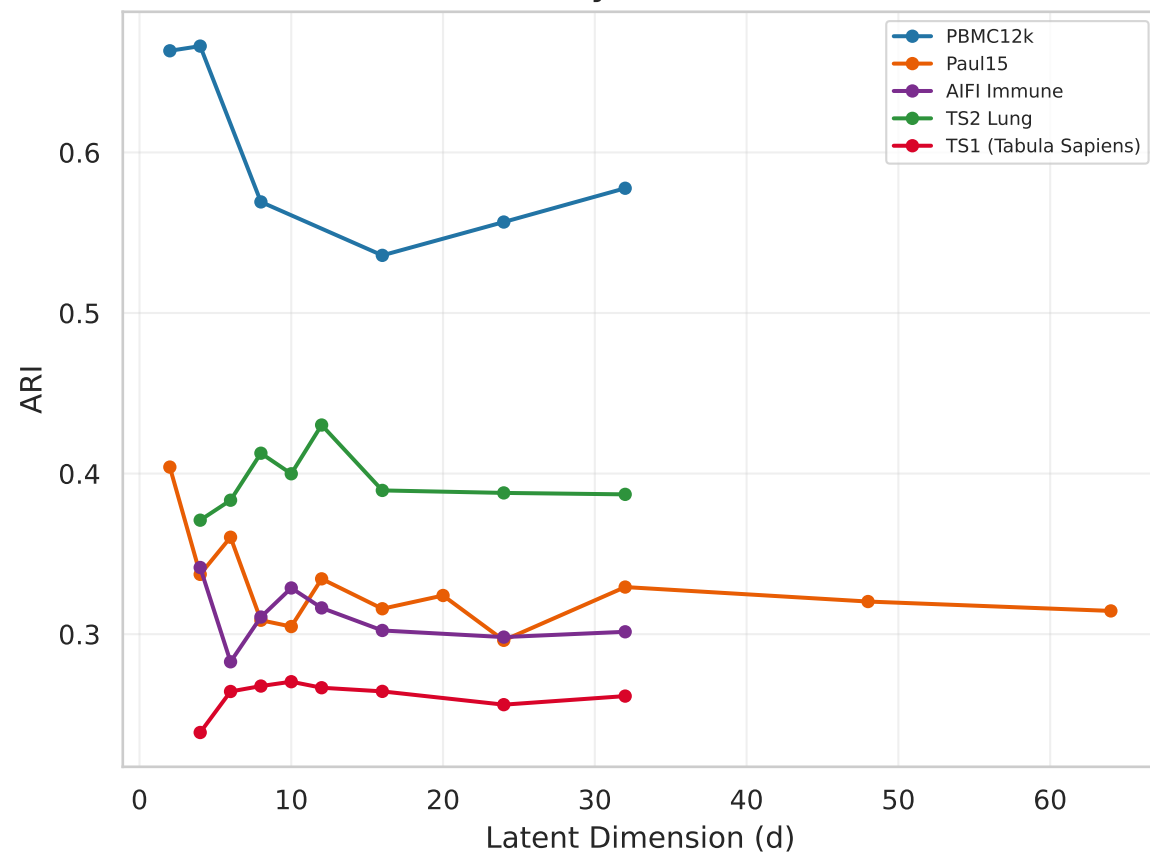
(C) ARI vs d by Dataset (scVI-NB)
