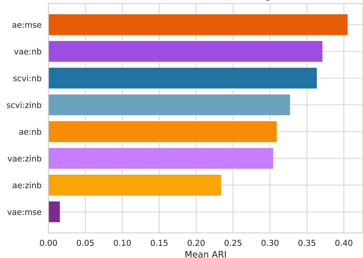
(B) Overall Model Ranking
