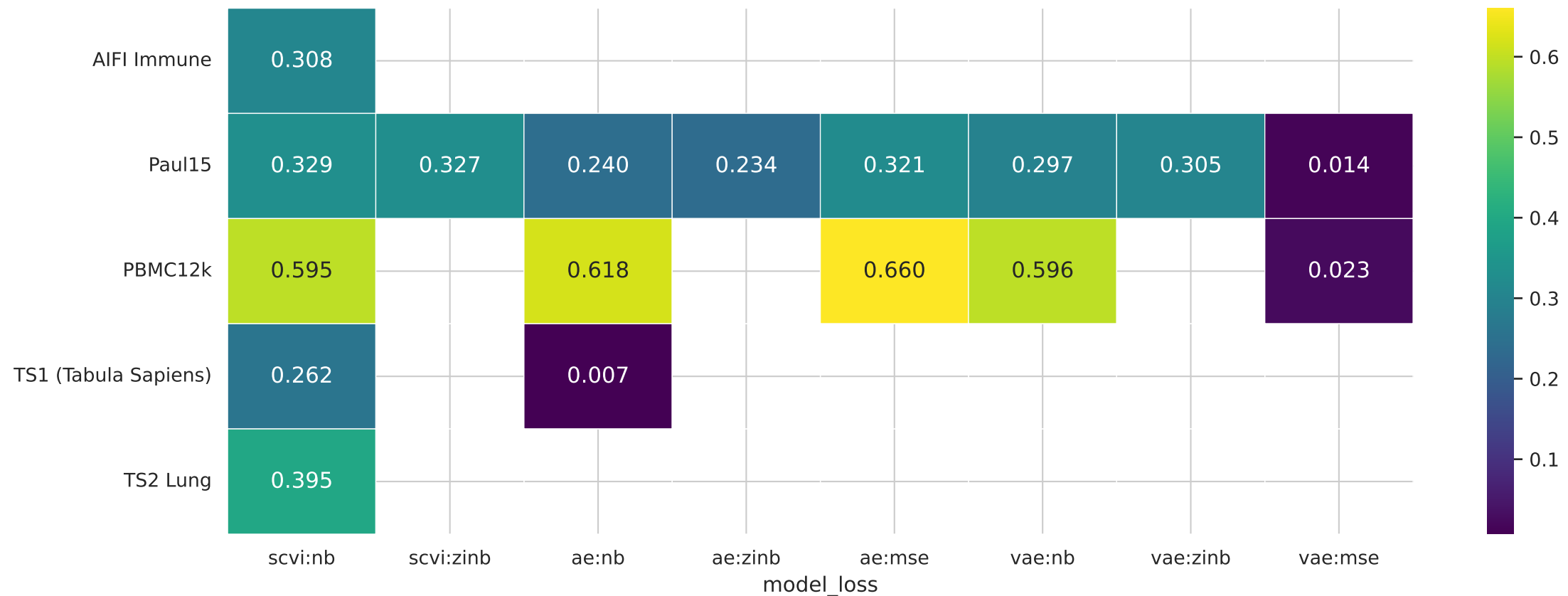
Mean ARI: All Datasets × Model/Loss Combinations
