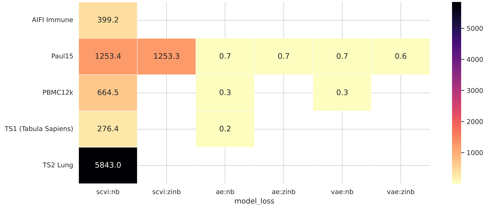
Mean Reconstruction Loss: Count-Likelihood Models
