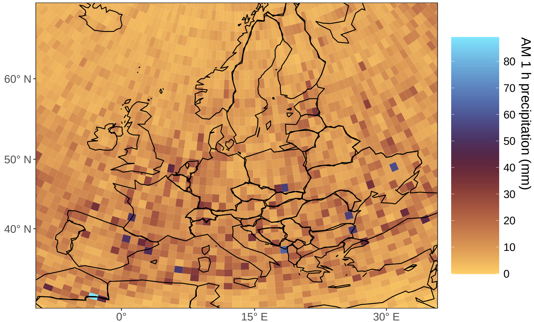
Annual maximum 1 h precipitation in 2005 for COSMO-crCLIM downscaling CNRM-CERFACS-CNRM-CM5
