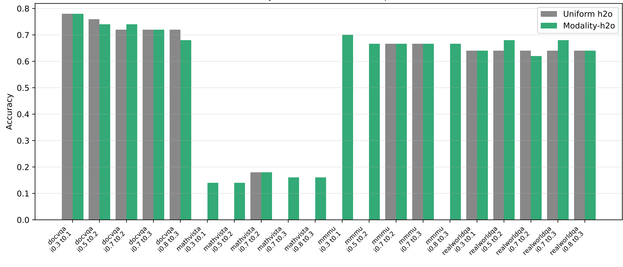
Modality-aware vs uniform compression
