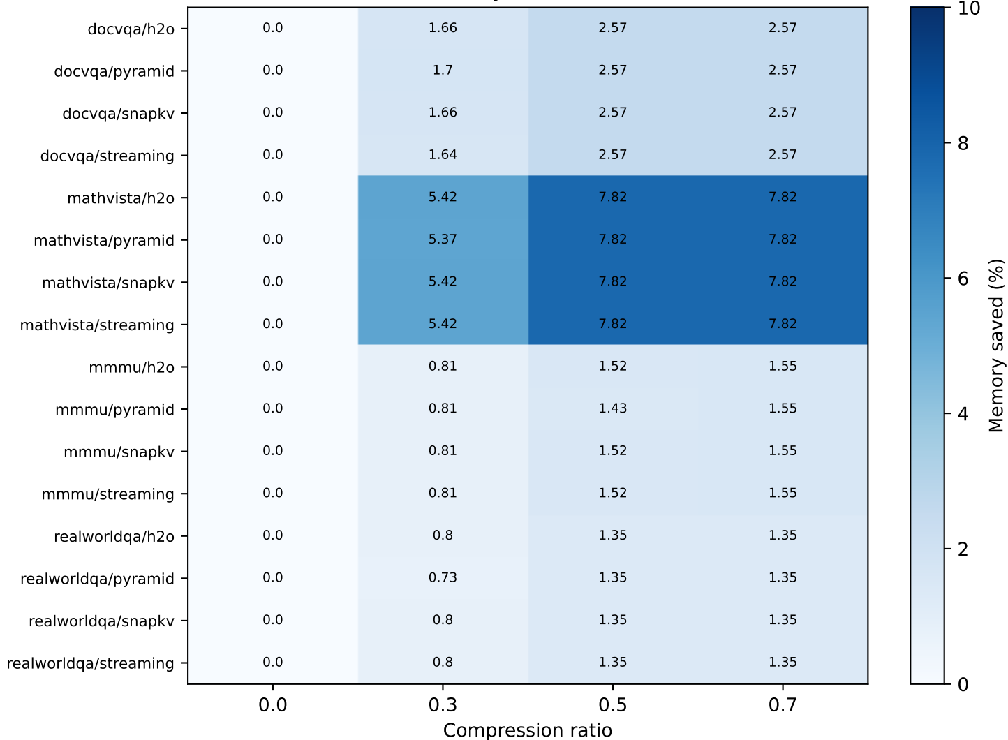
Peak GPU memory reduction vs. baseline
