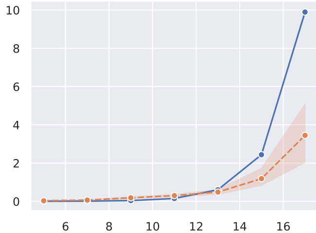
features=1
