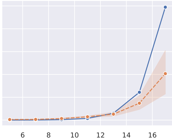
features=3
