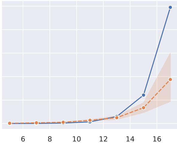
features=2
