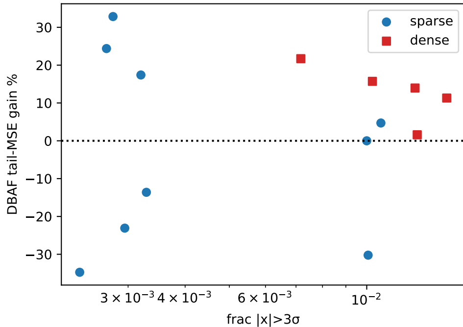
Tail ( |x| > T ) of distribution
