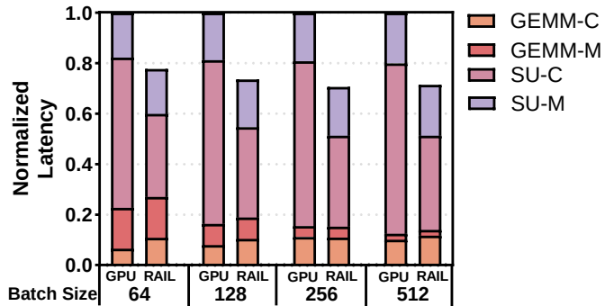
(a) Latency breakdown
