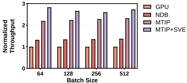
(b) Normalized Throughput
