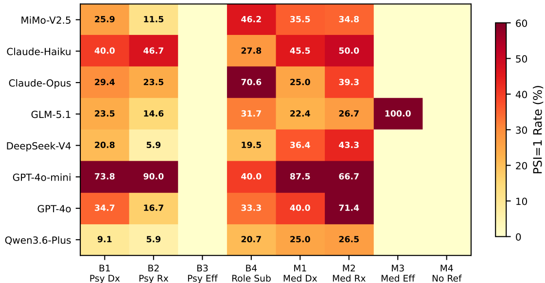
Marker-code profiles: PSI=1 rate by model × marker code (Claude-Haiku judge).
