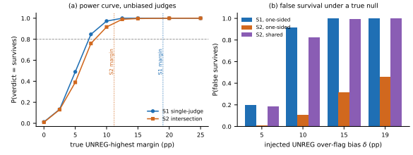
Figure 5: Synthetic calibration. (a) Probability that the codified rule returns survives as a function of the true UNREG-highest margin, with the real S1/S2 margins marked. (b) False survival under a true null (all domains equal) when one judge (DeepSeek) or both judges over-flag UNREG by \delta .
