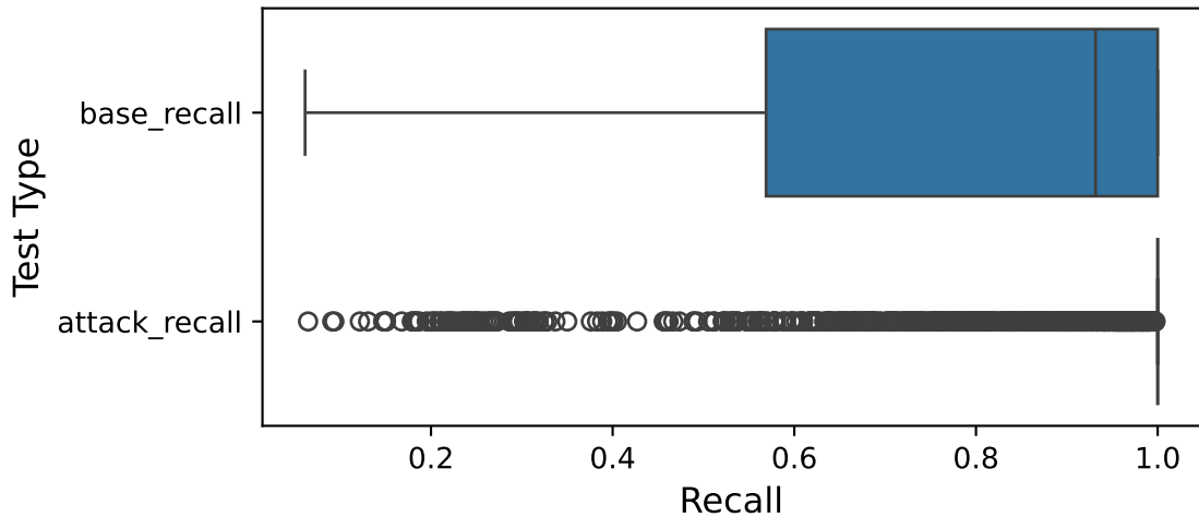
Comparison of Recall: Baseline versus Attack
