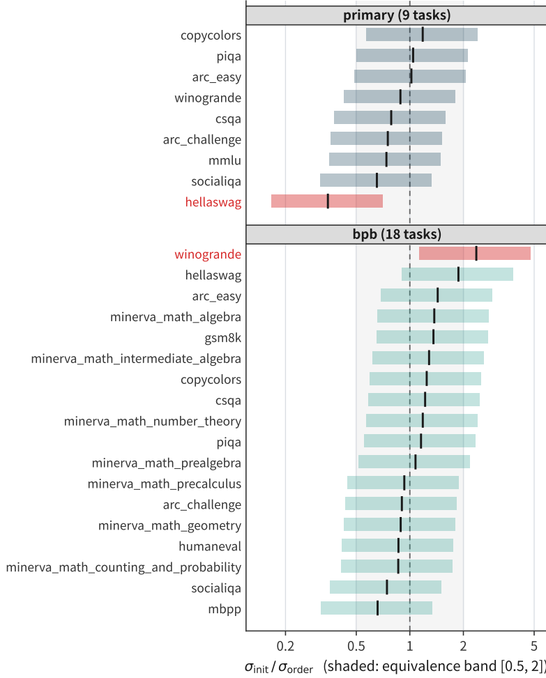
Figure 4: Source equivalence, task by task. Per-task \sigma_{\text{init}} / \sigma_{\text{order}} with CIs vs. the [0.5, 2] band (shaded): no CI fits inside; the two tasks excluding 1 do so in opposite directions, and neither survives Bonferroni control (Table 9).
