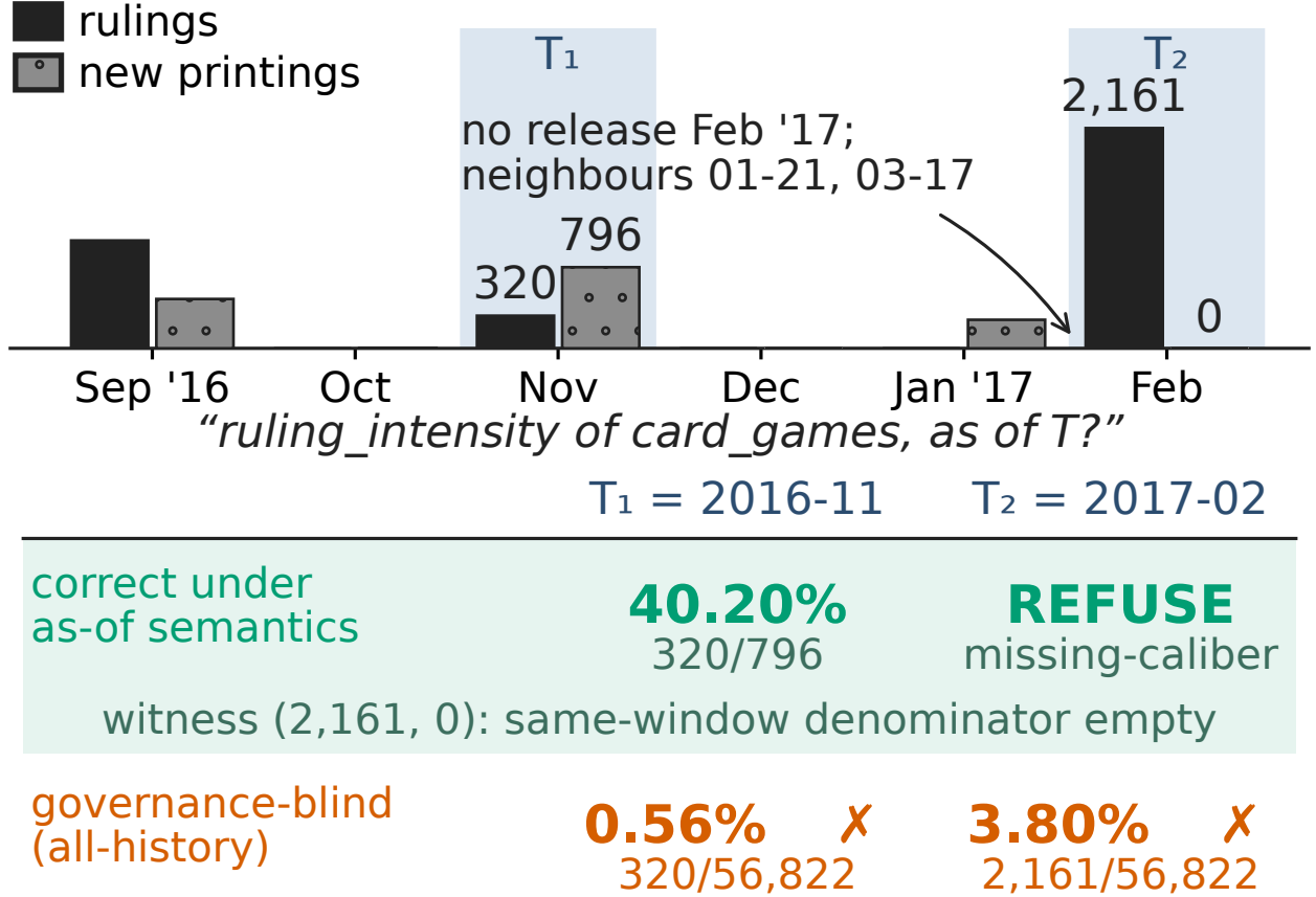
Figure 1: The as-of gap. Under the graph version in effect at the declared instant ( v_1 of card_games ; v_2 commits 2017-09-28), ruling_intensity binds its numerator on rulings.date and its denominator on sets.releaseDate under same_valid_time_window . At T_2 the numerator holds 2,161 rulings but the same-window denominator is empty inside validity, so the governed answer is \perp_{MC} , witnessed by a probe re-evaluating to 0 (panels and fractions on the figure).
