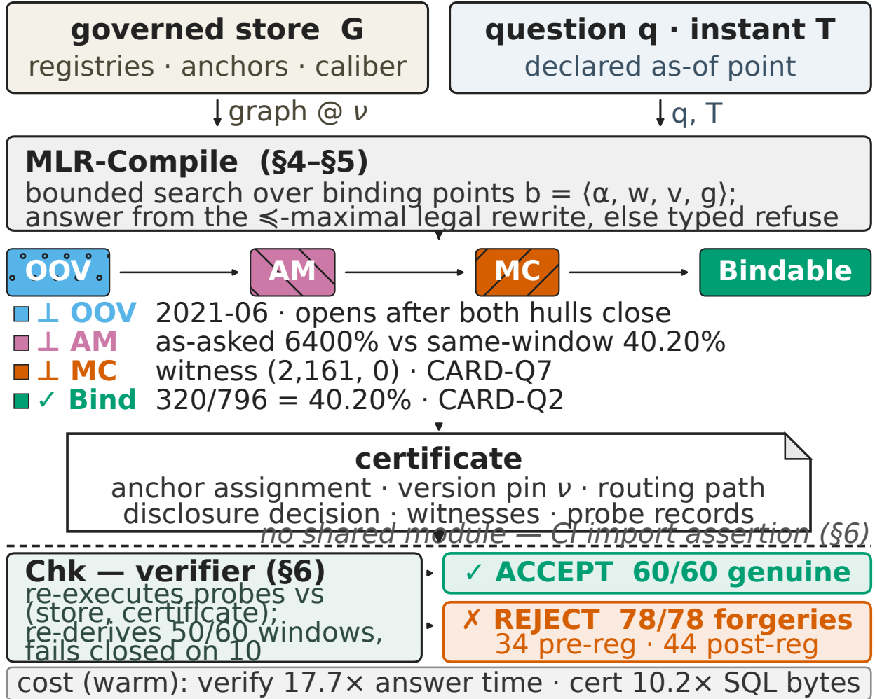
Figure 2: From question to independently checkable decision. MLR-COMPILER binds (q, T) ; the guard chain fires in the frozen order OOV \rightarrow AM \rightarrow MC , so every request exits Bindable or as one typed refusal (a worked instance under each exit; the full walk is in [33]). Both ship as a certificate — the only object crossing to Chk, which shares no compiler module and re-executes the probes: 60/60 genuine accept, 78/78 forgeries reject (§7.5), at a median 17.7× the answering time and 10.2× its bytes.
