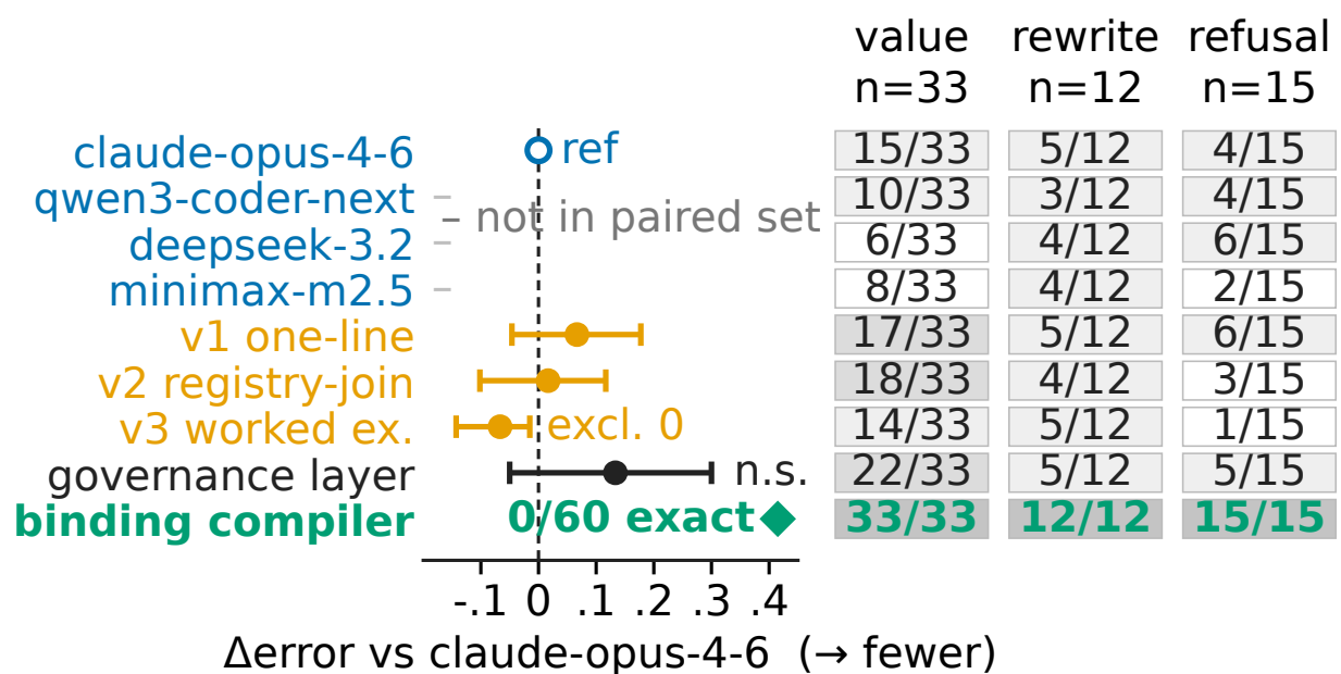
Figure 3: Effects with uncertainty (left: paired error reduction vs the reference, cluster-bootstrap 95% CIs over nine databases; only v3’s excludes zero, wrong-signed) and accuracy by gold form (right: the three denominators partition the true denominator of 60), in the row order of Table 4.
