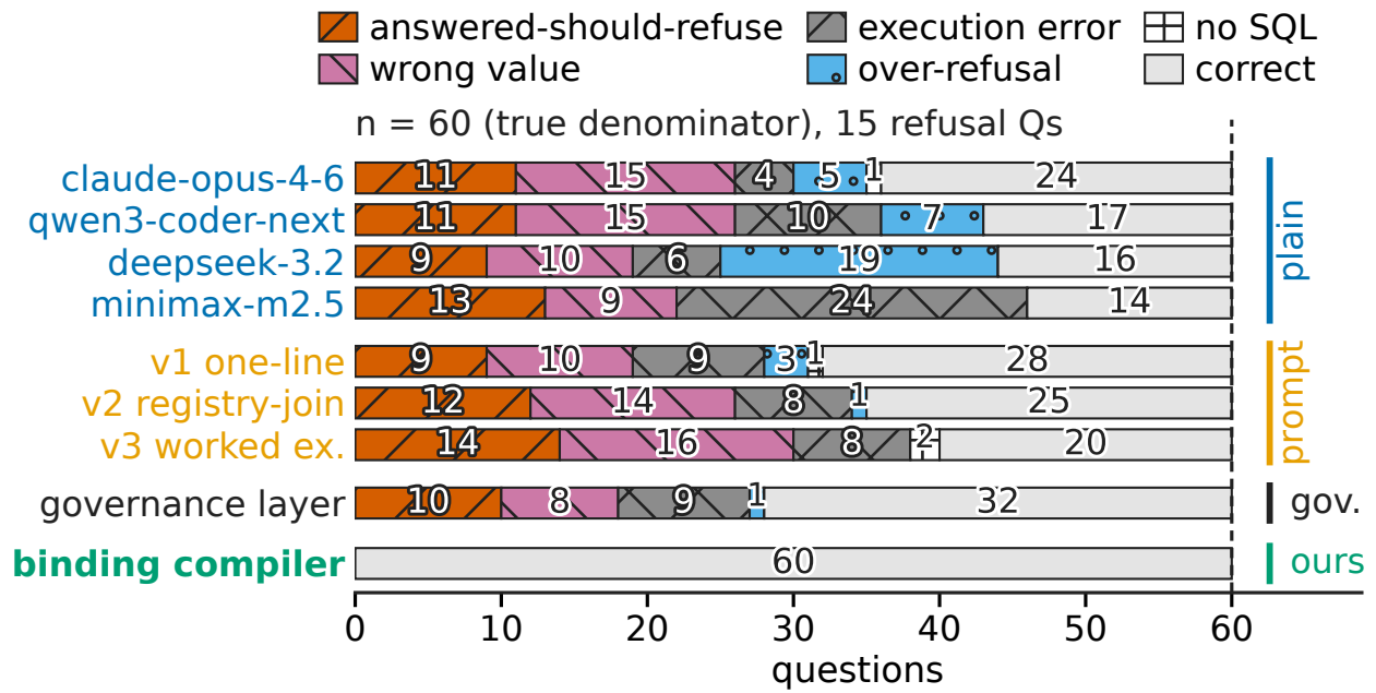
Figure 3: Failure taxonomy in the row order of Table 4: each bar stacks to the true denominator of 60, every non-empty segment prints its count. Wrong value includes a wrong window or version; no SQL is neither an answer nor a refusal.
