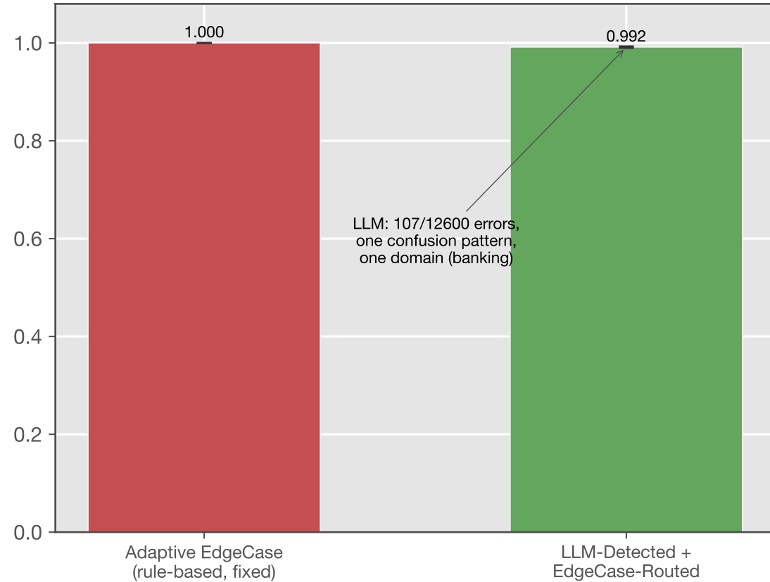
Mitigation Accuracy (same routing table, different detector)
