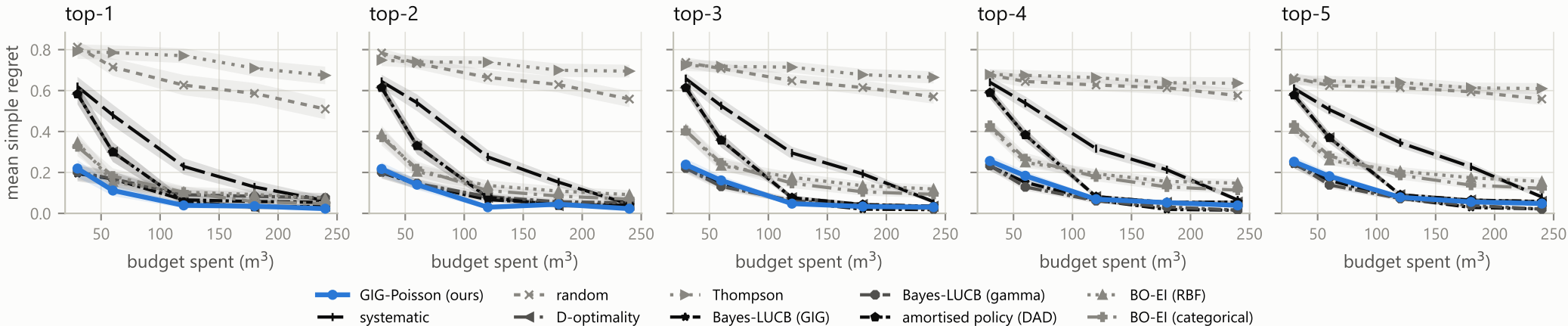
Bulk sampling, priors from 20 blocks per facies (acquisitions): top-m regret (shaded: \pm 1 s.e. over 50 runs)
