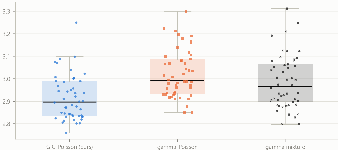
Bulk sampling, priors from 20 blocks per facies (models): held-out NLPD at the full budget (240 m 3 ), 50 runs
