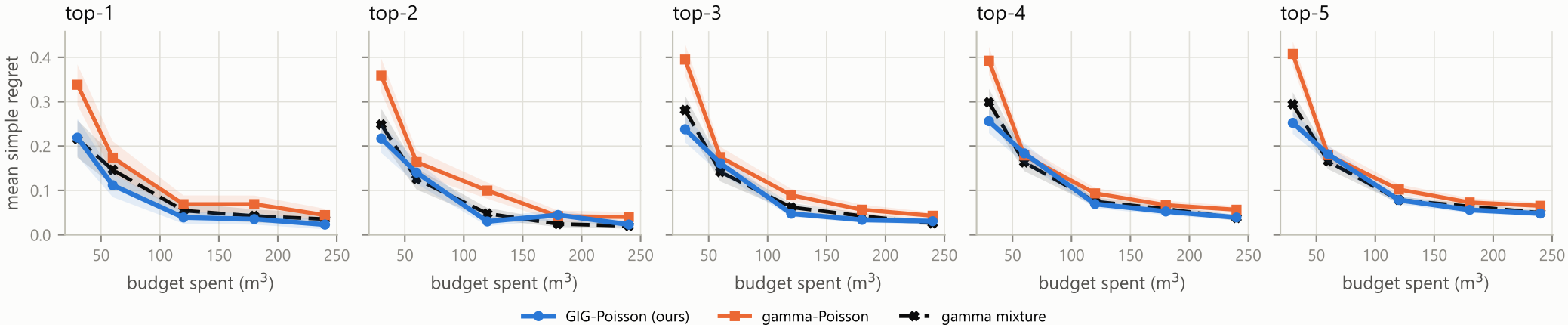
Bulk sampling, priors from 20 blocks per facies (models): top-m regret (shaded: \pm 1 s.e. over 50 runs)
