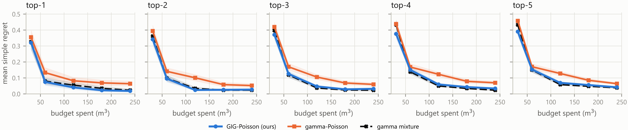
Bulk sampling, priors from 200 blocks per facies (models): top-m regret (shaded: \pm 1 s.e. over 50 runs)
