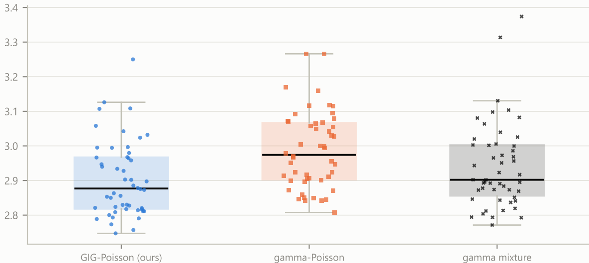
Bulk sampling, priors from 40 blocks per facies (models): held-out NLPD at the full budget (240 m 3 ), 50 runs
