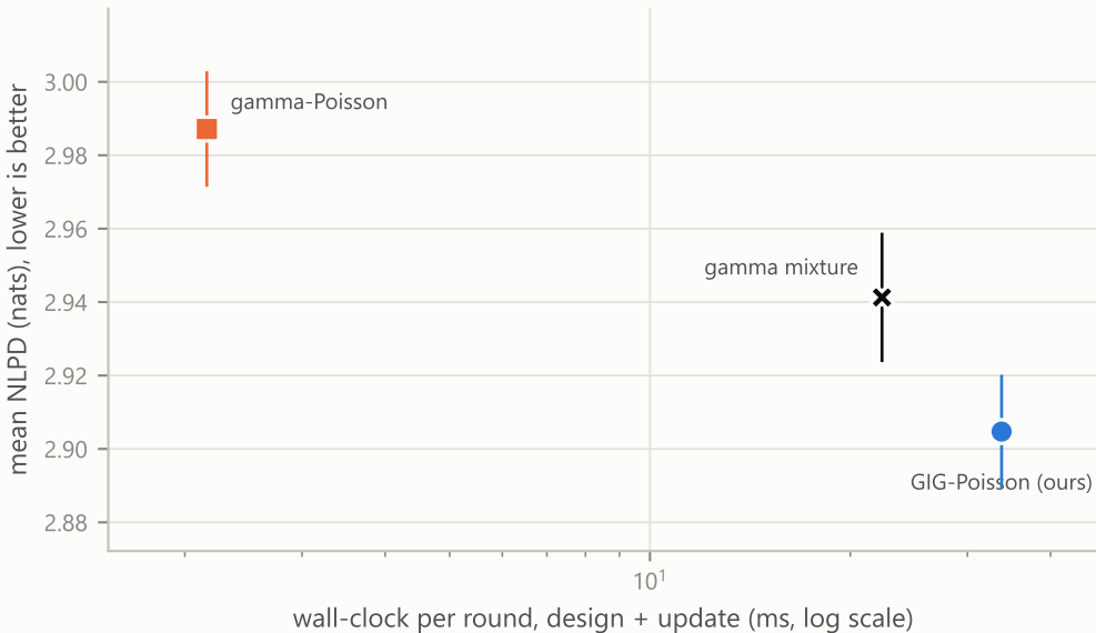
Bulk sampling, priors from 40 blocks per facies (models): accuracy against cost, 50 runs
