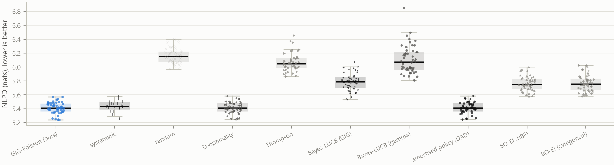
Gamma-ray survey, priors from 20 sources per class (acquisitions): held-out NLPD at the full budget (120 Ms), 50 runs
