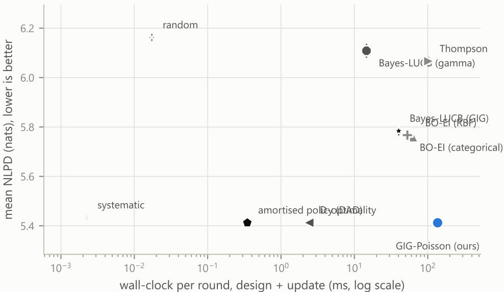
Gamma-ray survey, priors from 20 sources per class (acquisitions): accuracy against cost, 50 runs
