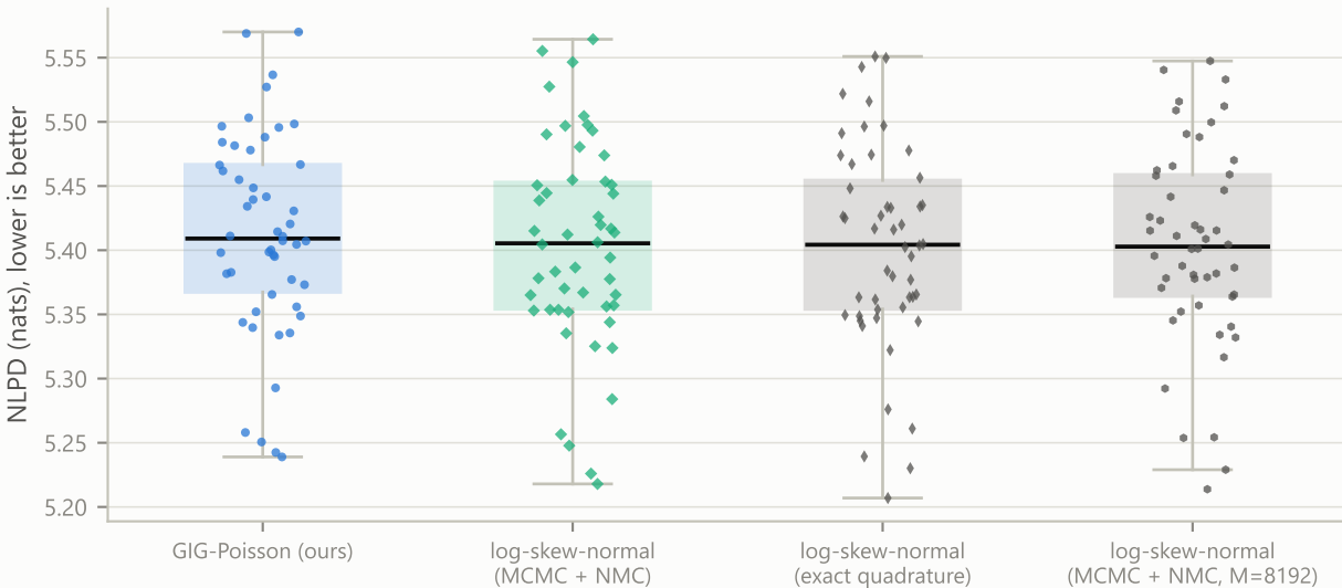
Gamma-ray survey, priors from 20 sources per class (appendix_lsn): held-out NLPD at the full budget (120 Ms), 50 runs
