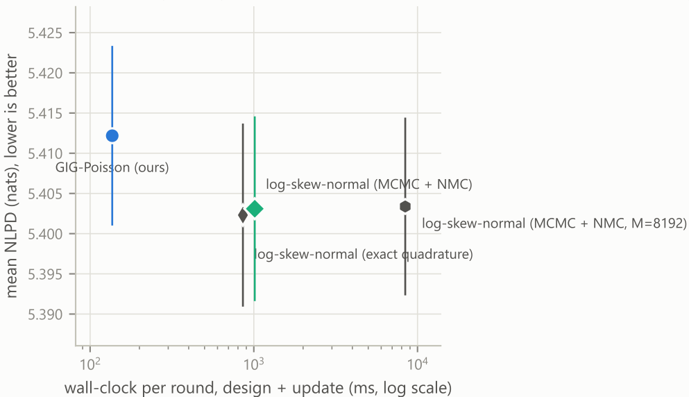
Gamma-ray survey, priors from 20 sources per class (appendix_lsn): accuracy against cost, 50 runs
