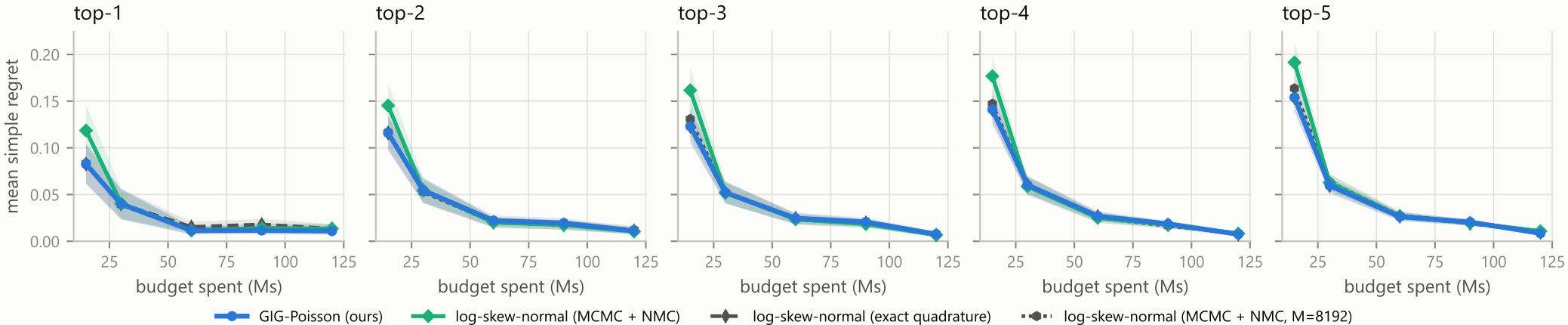
Gamma-ray survey, priors from 20 sources per class (appendix_lsn): top-m regret (shaded: \pm 1 s.e. over 50 runs)
