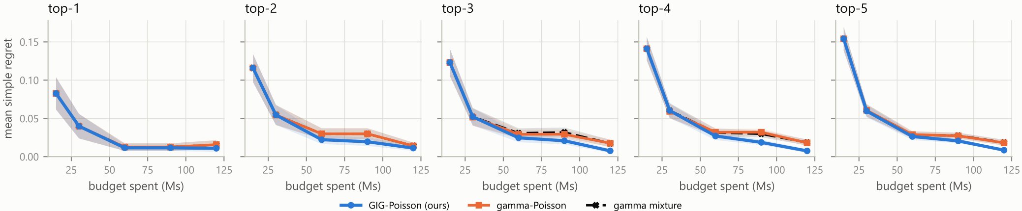
Gamma-ray survey, priors from 20 sources per class (models): top-m regret (shaded: \pm 1 s.e. over 50 runs)
