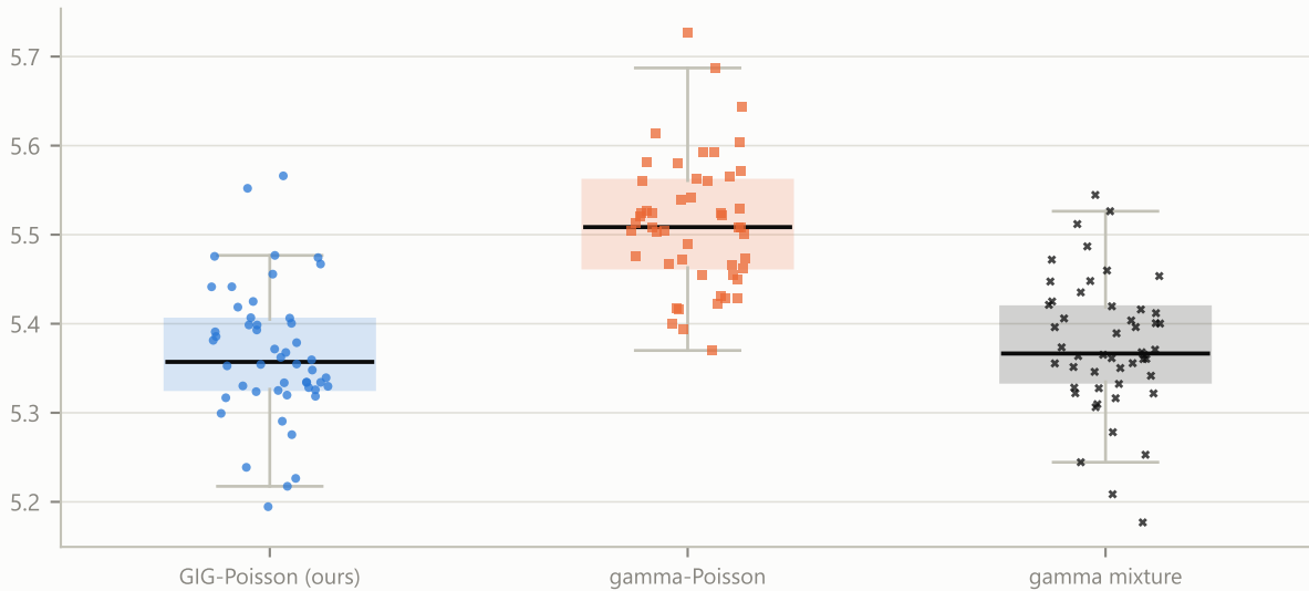
Gamma-ray survey, priors from the full catalogue half (models): held-out NLPD at the full budget (120 Ms), 50 runs
