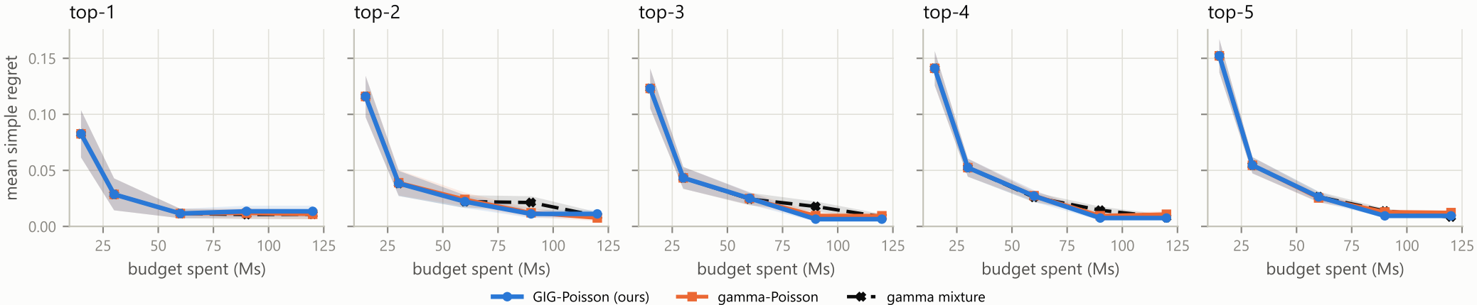
Gamma-ray survey, priors from the full catalogue half (models): top-m regret (shaded: \pm 1 s.e. over 50 runs)
