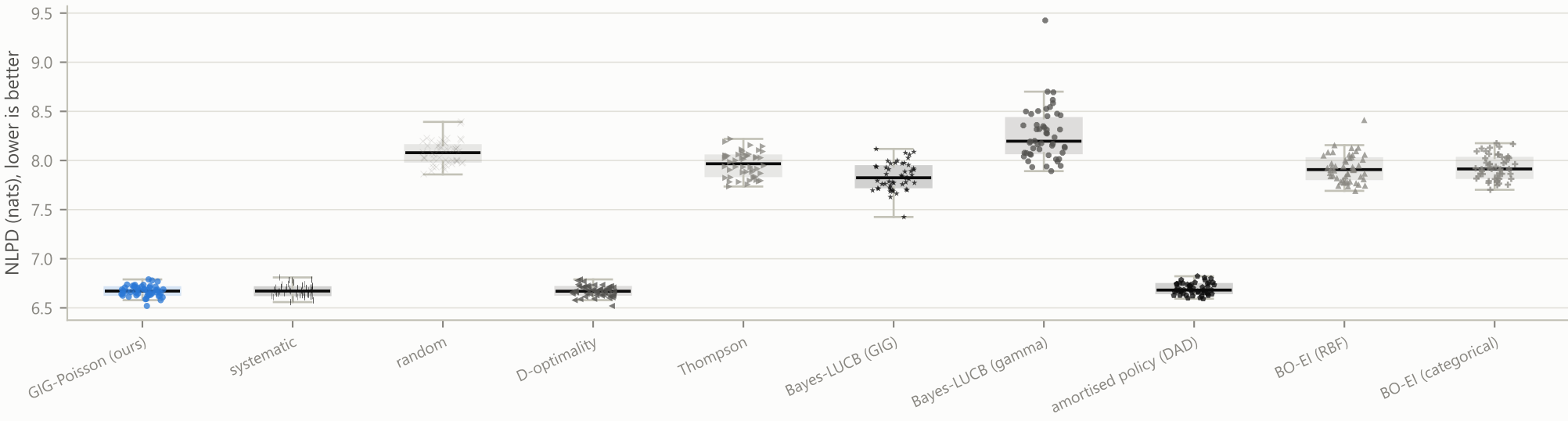
Hard X-ray follow-up, priors from 20 sources per class (acquisitions): held-out NLPD at the full budget (120 ks), 50 runs
