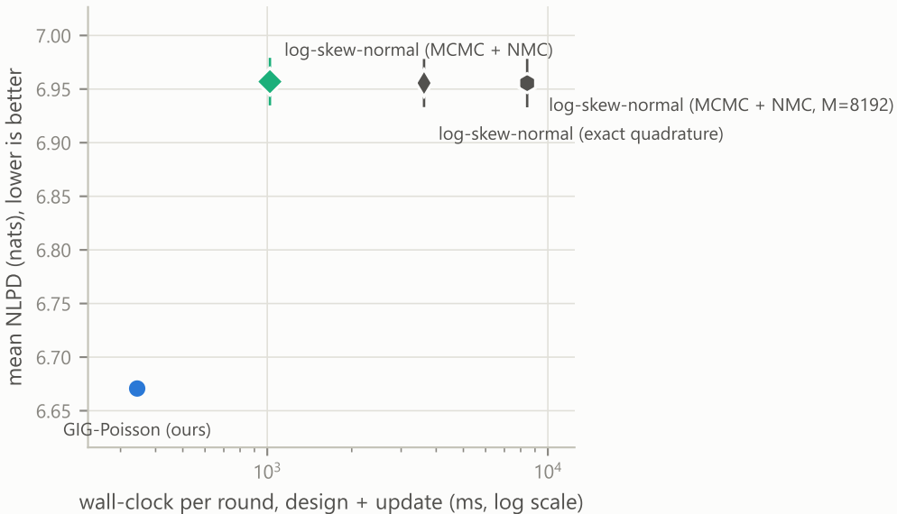
Hard X-ray follow-up, priors from 20 sources per class (appendix_lsn): accuracy against cost, 50 runs
