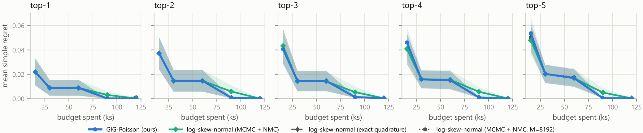
Hard X-ray follow-up, priors from 20 sources per class (appendix_lsn): top-m regret (shaded: \pm 1 s.e. over 50 runs)
