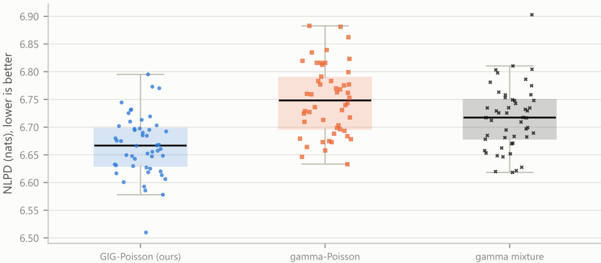
Hard X-ray follow-up, priors from 40 sources per class (models): held-out NLPD at the full budget (120 ks), 50 runs
