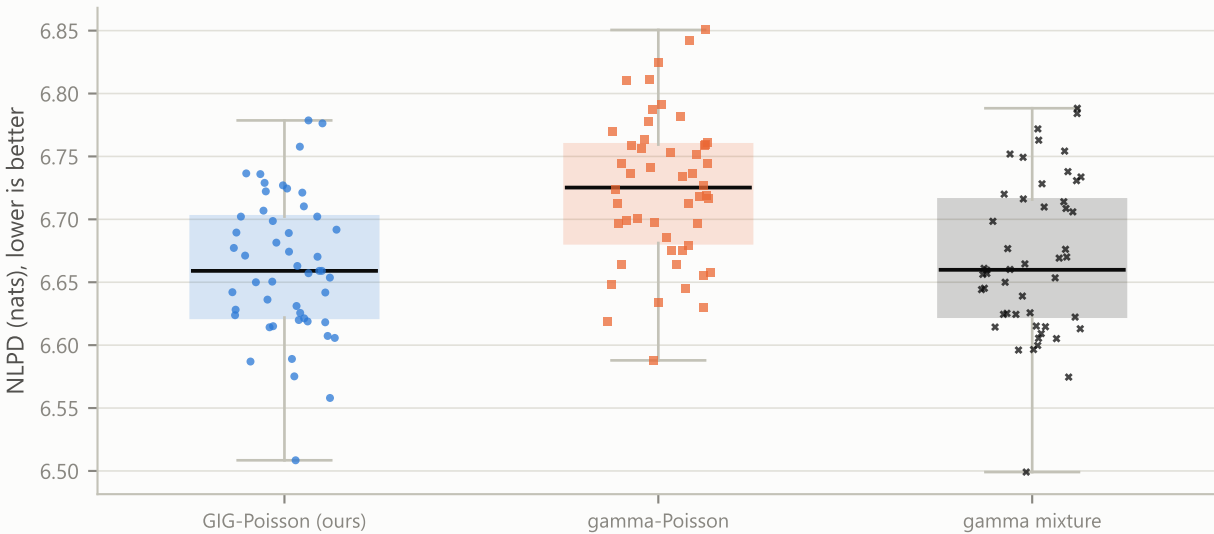
Hard X-ray follow-up, priors from the full catalogue half (models): held-out NLPD at the full budget (120 ks), 50 runs
