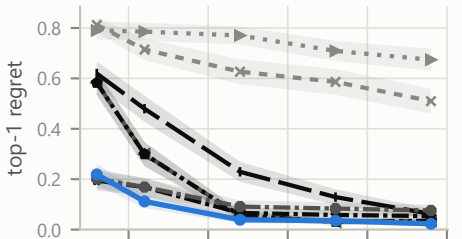
Diamond bulk sampling
