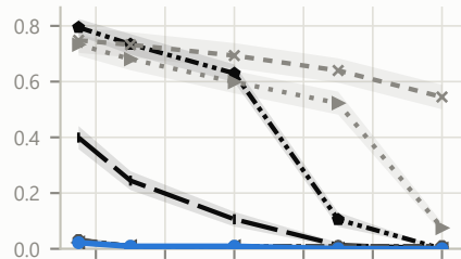
Hard X-ray follow-up (Swift-BAT)
