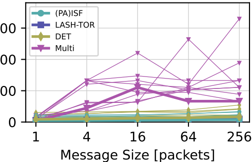
WSI (Interleaved)
