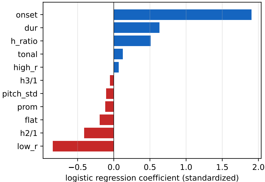
Feature importance (+ = whistle-like)
