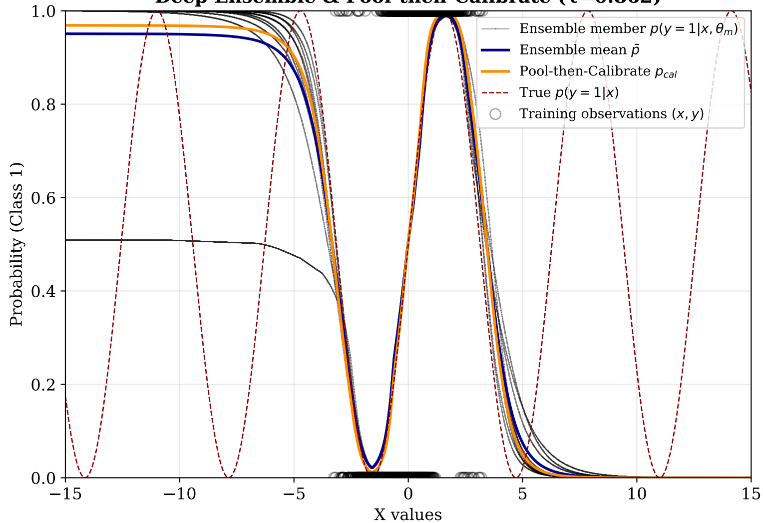
Deep Ensemble & Pool-then-Calibrate ( \tau=0.862 )
