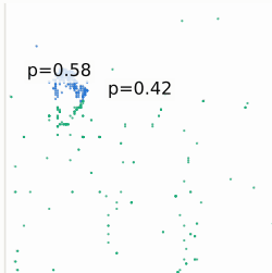
mixture components
