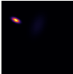
persistence-weighted density
