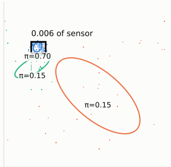
Gaussian mixture
