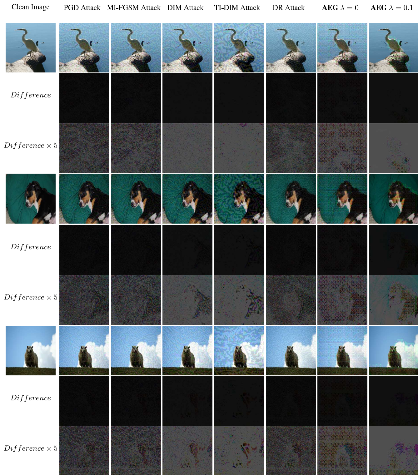
Figure 2: Example clean images and adversarial images generated by different attack methods.
