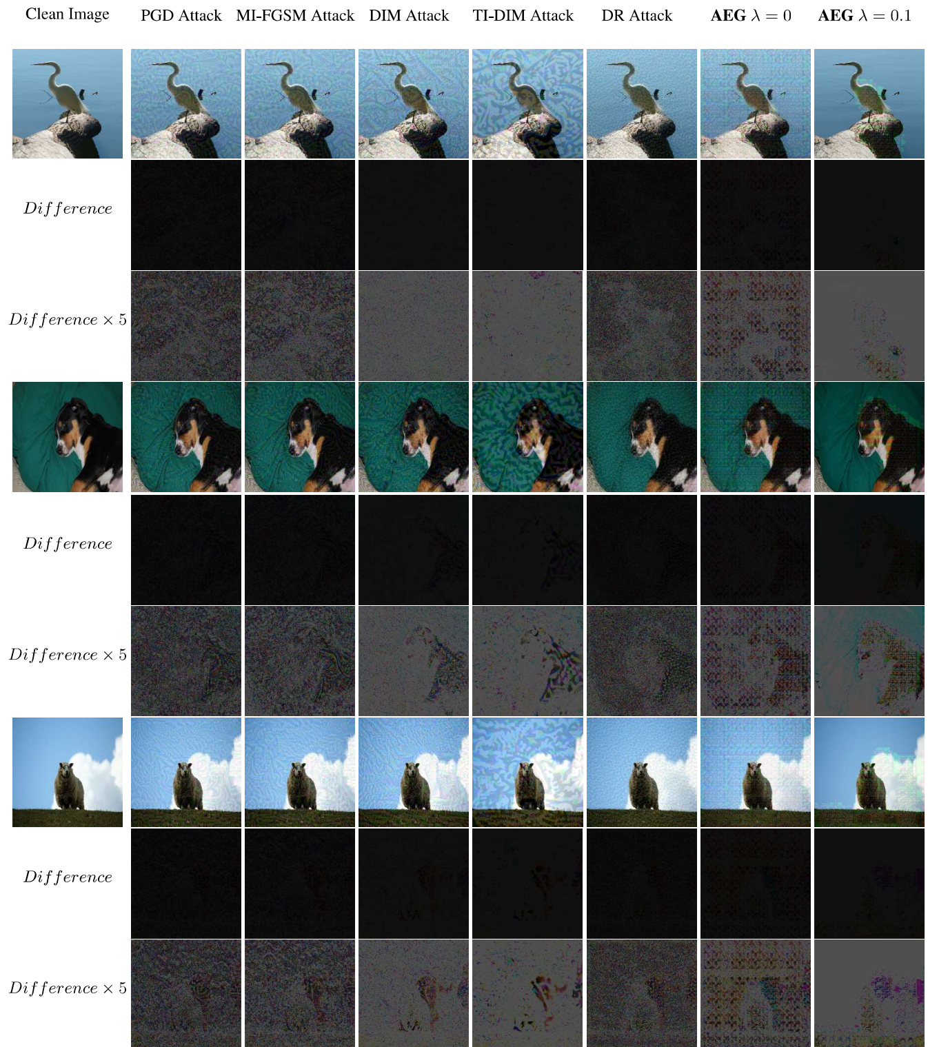
Figure 2: Example clean images and adversarial images generated by different attack methods.
