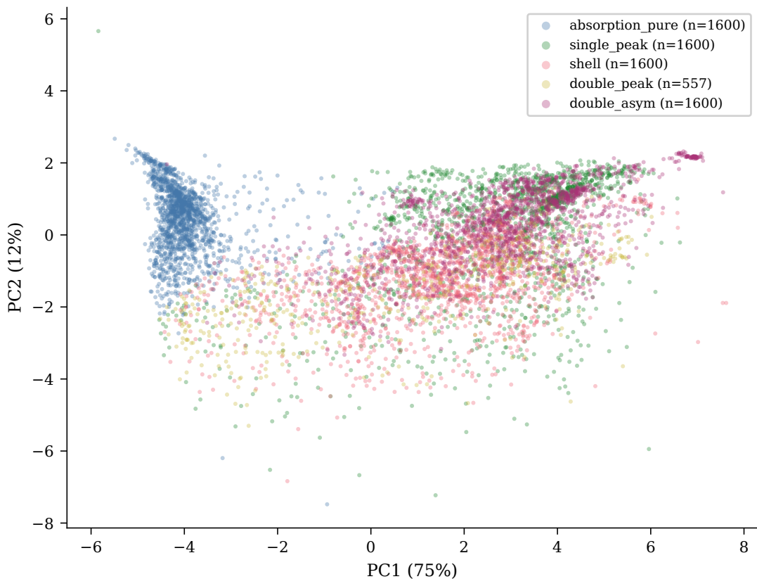
PCA of BeMAE embeddings, coloured by H \alpha morphology
