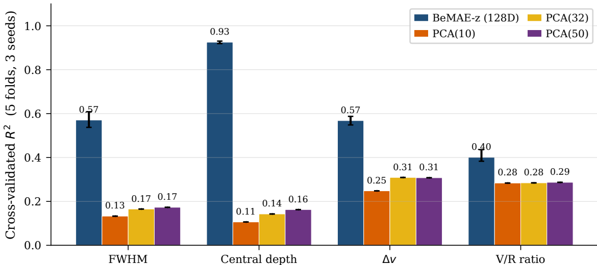
SpecProbe: BeMAE-z vs PCA on four spectral features
