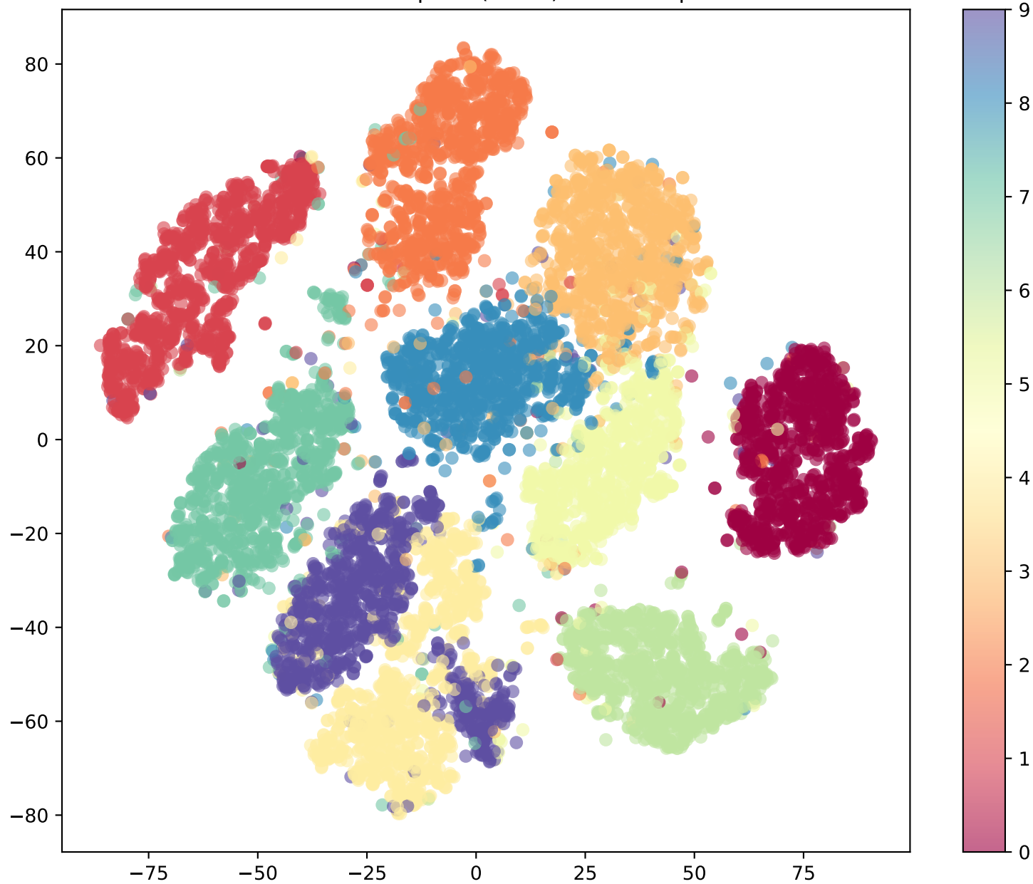
TSNE of Latent Space (d=20) after 50 epochs
